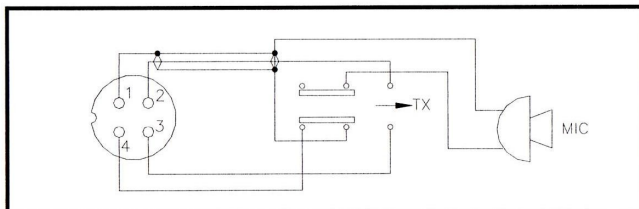
Fig. 3. Your transceiver microphone schematic
