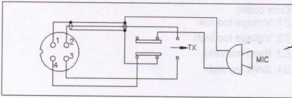
Fig. 1 Your transceiver microphone schematic.
