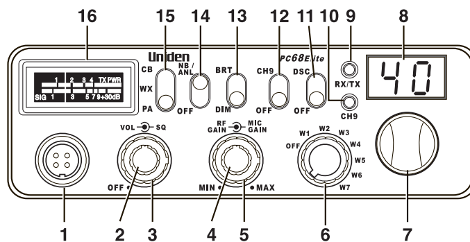
FRONT VIEW - PC68 Elite BACKLIGHTED PANEL
