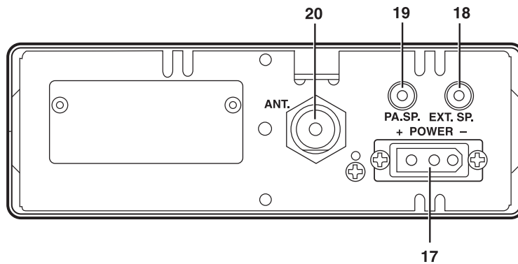
REAR VIEW
